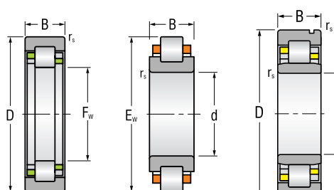
Special single-row cylindrical roller bearings
