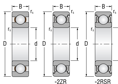
Single-row deep groove ball bearings
