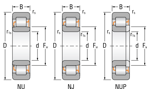
Cylindrical roller bearings
