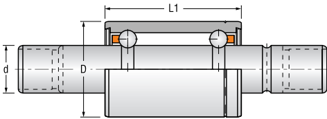
Special double-row bearings type „K“
