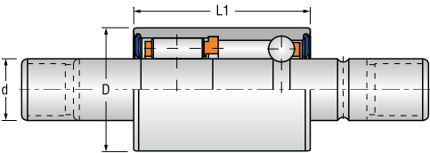
Special double-row bearings type „R“
